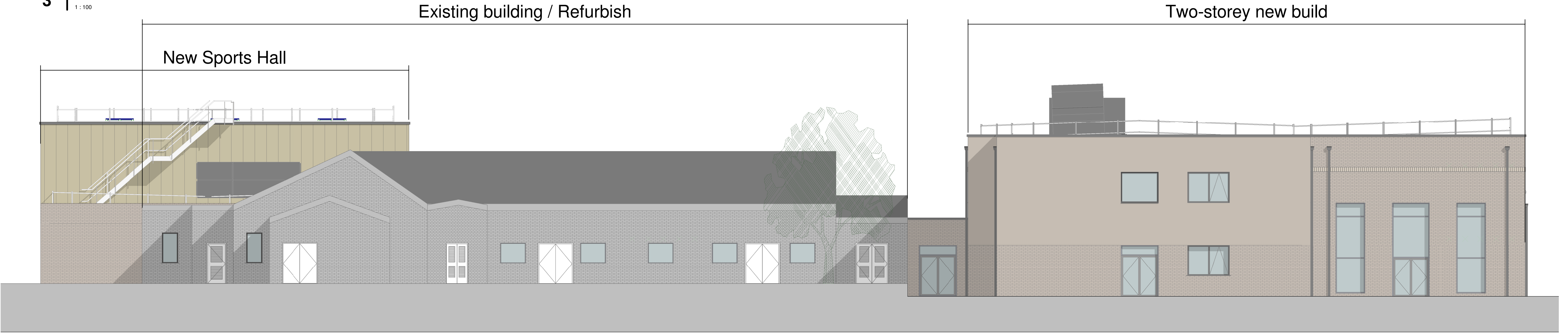
4 | West Elevation 1:100
