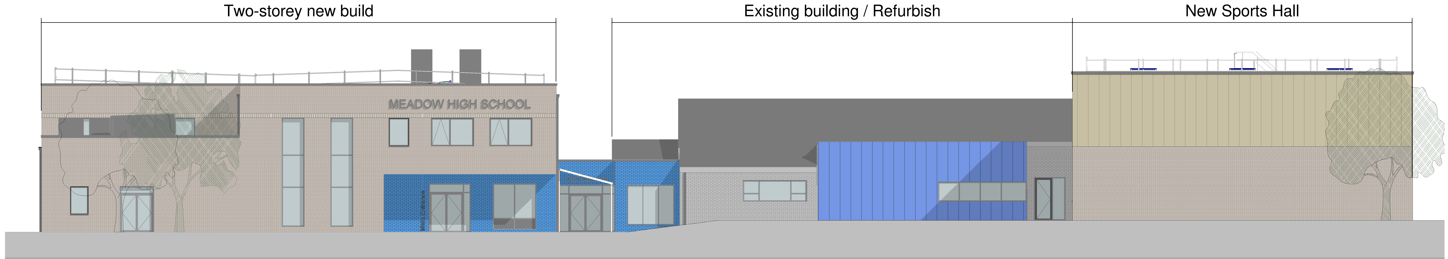
3 | East elevation 1:100
